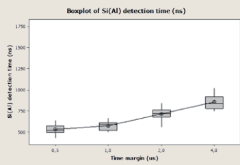
Fig. 8. Effect of the selected “Time margin” on the detection time. Target Si(AI). “Voltage margin” was set at 100V.
