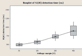
Fig. 7. Effect of the selected “Voltage margin” on the detection time. Target Si(AI). “Time margin” was set at 1µs.
