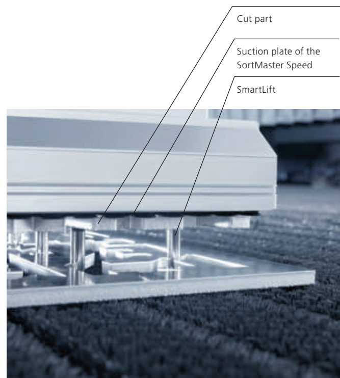
Process-reliable part removal: SortMaster Speed and SmartLift.
