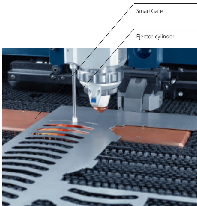
Parts are fixed between the ejector cylinder and the SmartGate, and are therefore removed with maximum process reliability.
