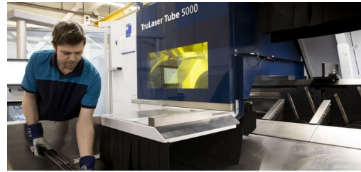
<p><span lang="EN-US">The TruLaser Tube 5000 can be unloaded manually, but it can also operate without an operator. In that case, an unloading station from TRUMPF partner transfluid® takes over this task. </span></p>
