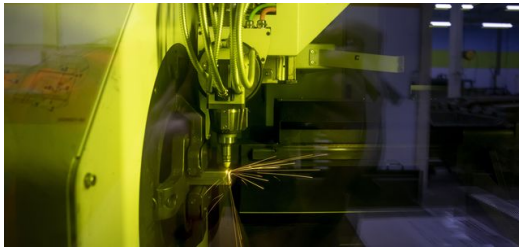
<p><span lang="EN-US">The TruLaser Tube 5000 laser tube cutting machine cuts all the necessary openings in the tube. </span></p>
