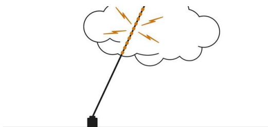
Discharging storm clouds 1: triggering lightning within a cloud. – Gernot Walter
