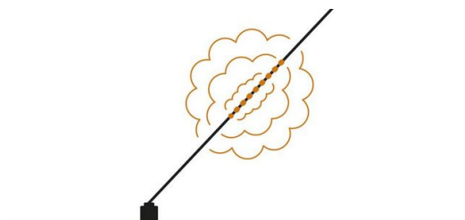
Making clouds. – Gernot Walter
