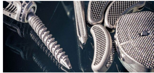
<p>The implants consist of a fine mesh. This fuses more quickly with the bone. <span lang="DE">Only the laser can print it.</span></p>
