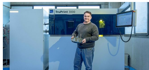
<p>The TruPrint 3000 is equipped with the multilaser option. With two 500-watt lasers, Tsunami builds the cages twice as fast using the laser metal fusion process.</p>
