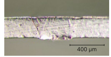
Heat conduction welding of copper foil with v = 10 \text{ m/min} , seam surface and cross section.
