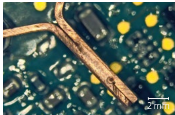
Welding of electronic components with minimum spatter formation thanks to green wavelength.
