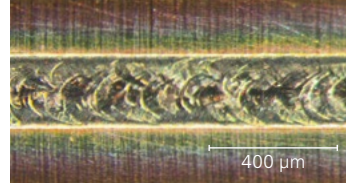
Heat conduction welding of copper foil with v = 10 \text{ m/min} , seam surface and cross section.
