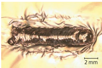
Welding of battery foil stacks consisting of 100 copper foils with TruDisk 2021. Left: Regular seam surface without ejections. Right: Cross section of the poreless weld seam with large joint area.
