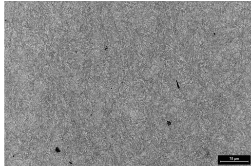
Figure 9: Microstructure of Dievar: AM_A_W_W_42-44_HRC
