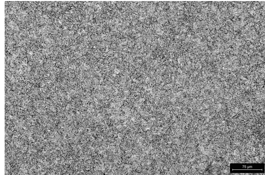
Figure 13: Microstructure of H13: AM_A_W_W_W_44-46_HRC
