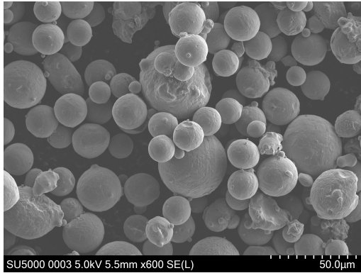
Figure 11: H11 powder by Höganäs. PSD: 10-45 μm. SEM magnification: 600x.
