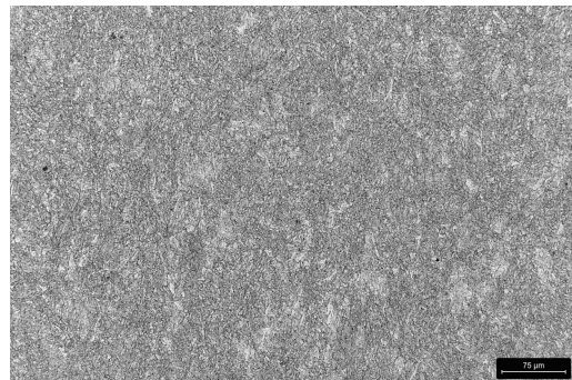
Figure 14: Microstructure of H13: AM_A_W_W_W_52-54_HRC
