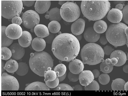
Figure 7: Dievar powder by Uddeholm. PSD: 20-53 μm. SEM magnification: 600x.
