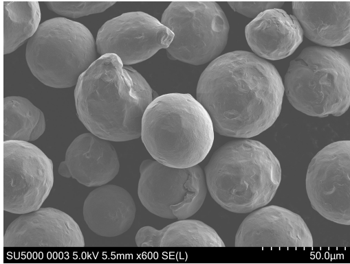
Figure 16: M2 powder by Höganäs. PSD: 20-53 µm. SEM magnification: 600x.
