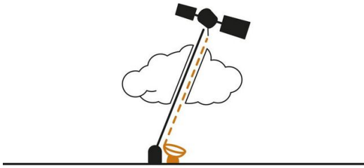
<p><span lang="EN-US">Drilling holes in clouds. </span></p> – Gernot Walter
