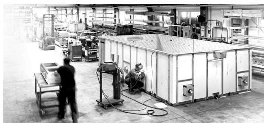
In one piece: Pools with standard dimensions are fully finished at Gassner and transported to the installation site on flatbed trucks. Picture: Niels Schubert
