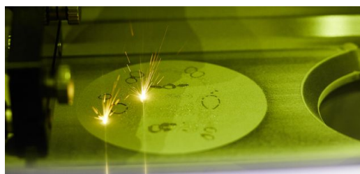
Multiple or single laser? The optimum number depends on the size of the building chamber.
