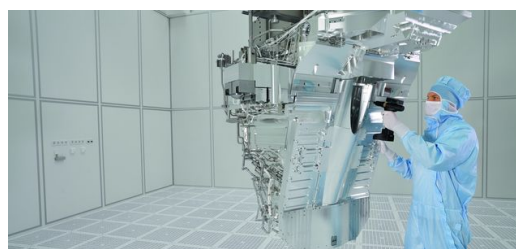
EUV optics system from Zeiss.
