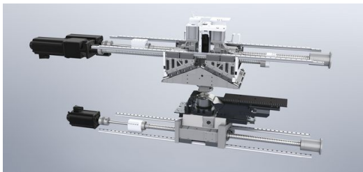
Small parts are reliably removed // Subsequent sorting of good and waste parts is no longer needed // Fewer scratches on good parts // Sheet thicknesses up to 6 mm (Image: Electronic Publishing Stefan Berner GmbH)
